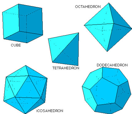
the 5 Platonic Solids
