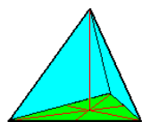
trigonal pyramid
