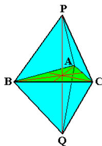
trigonal bipyramid
